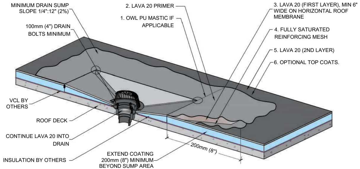
ISOMETRIC SECTION
