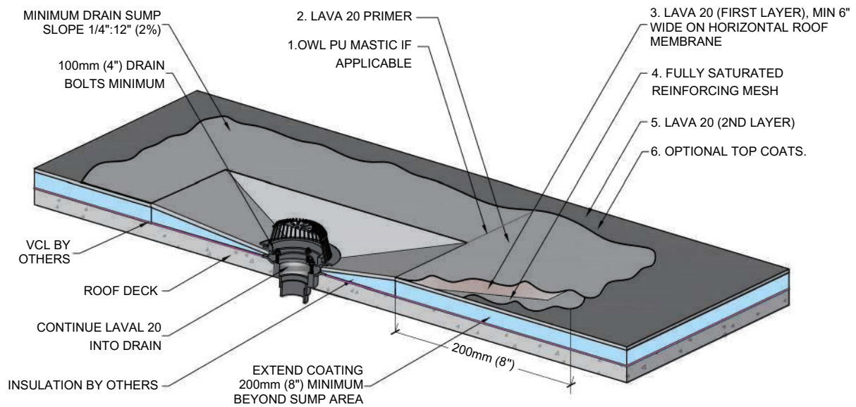
ISOMETRIC SECTION
